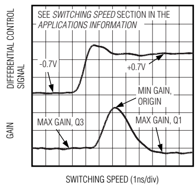
SWITCHING SPEED
