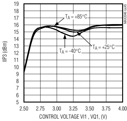
IIP3 vs. CONTROL VOLTAGE (VI1 = VQ1)
